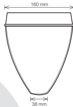
Mustang Exit Ceiling Mounted (Double Sided) SIDE VIEW
