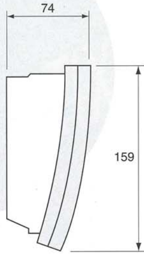
Catalogue Numbers: Single Sided Surface-Wall WL 2160 Maintained 8W
